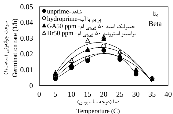
Figure 1- Predicted (solid lines) and observed (symbols) germination rates of camelina seeds under non-stress conditions at different temperatures and priming treatments, fitted using segmented, dent-like, and beta models.
