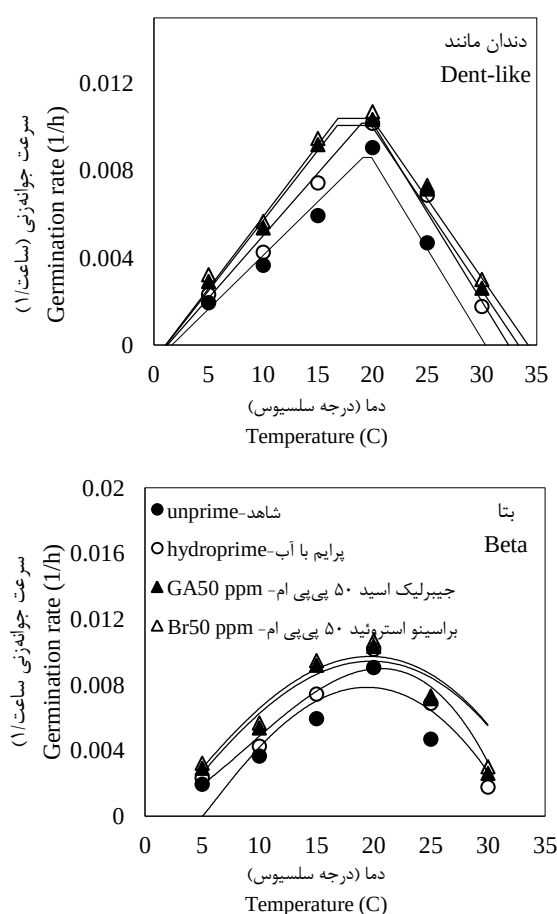
Figure 3- Predicted (solid lines) and observed (symbols) germination rates of camelina seeds at different temperatures and priming treatments using segmented, dent-like, and beta models under 200 mM salinity stress.
