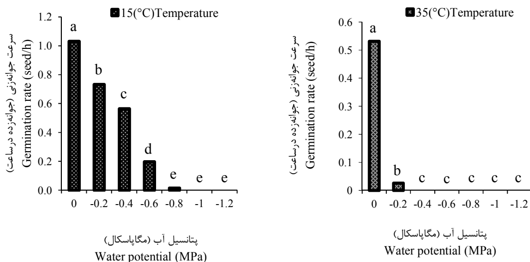
Fig. 2. The Effect of Water potential on germination rate of Fenugreek at 15 and 35 °C temperatures. In each section of this figure, the same letters indicate no significant difference based on the LSD test at the 5% level.
