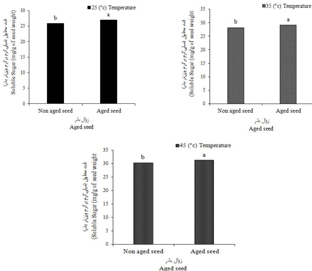
Fig. 6. The effect of seed aging on soluble sugar of Fenugreek at 25, 35, and 45 °C temperatures. In each section of this figure, the same letters indicate no significant difference based on the LSD test at the 5% level.
